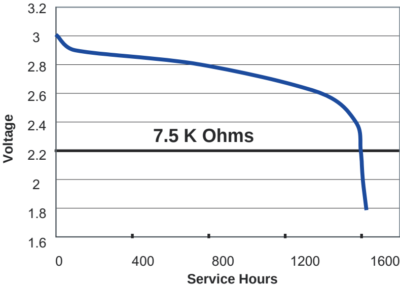
Typical Discharge Characteristics at 21°C (70°F)
